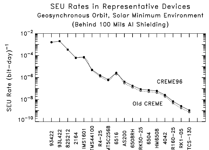
Fig. 3. SEU rates in representative devices at solar minimum, in geosynchronous orbit under 100 mils shielding, calculated with old CREME and CREME96.
