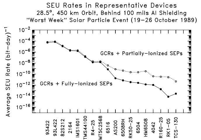
Fig. 8. Effect of solar particle ionic charge states on SEU rates in representative devices in 28.5° 450 km, behind 100 mils shielding.
